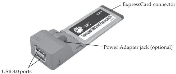
Figure 1: Layout
